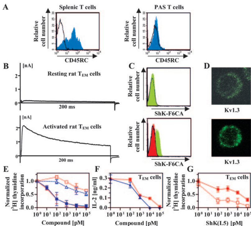
Fig. 3. ShK(L5) preferentially suppresses the proliferation of rat T_{\text{EM}} cells. A, CD45RC staining of rat splenic T cells (left) and PAS T cells (right) detected by flow cytometry. B, Kv1.3 currents exhibited by quiescent (top) and myelin antigen-activated (bottom) PAS T cells. C, flow cytometry profiles of ShK-F6CA-staining in quiescent (top) and myelin antigen-activated (bottom) PAS T cells. Unstained cells (black lines) and cells stained with ShK-F6CA (green filled). Competition of ShK-F6CA staining by unlabeled ShK(L5) is red-filled. D, confocal images of Kv1.3 immunostaining in quiescent (top) and myelin antigen-activated (bottom) PAS T cells. Statistical analysis was carried out using the Mann-Whitney U test. E, dose-dependent inhibition by ShK (blue) and ShK(L5) (red) of [^3\text{H}] thymidine incorporation by rat naive/ T_{\text{CM}} (open symbols) and T_{\text{EM}} (closed symbols) cells activated with Con A (1 \mu\text{g/ml} ). F, dose-dependent inhibition by ShK (blue) and ShK(L5) (red) of IL2 secretion by PAS T cells 7 h after stimulation with MBP. G, ShK(L5)-induced inhibition of myelin-antigen triggered [^3\text{H}] thymidine incorporation by PAS T cells (open symbols) is reversed by the addition of 20 units/ml IL2 (closed symbols).
